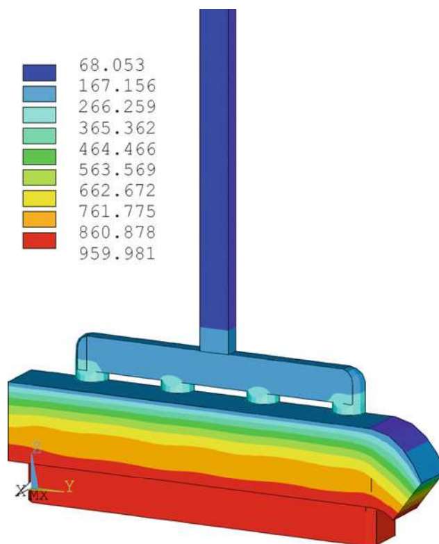
Fig. 2 500 kA half anode model temperature solution
