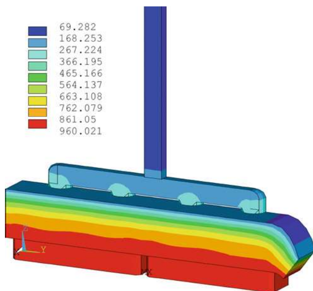
Fig. 6 650 kA half anode model temperature solution
