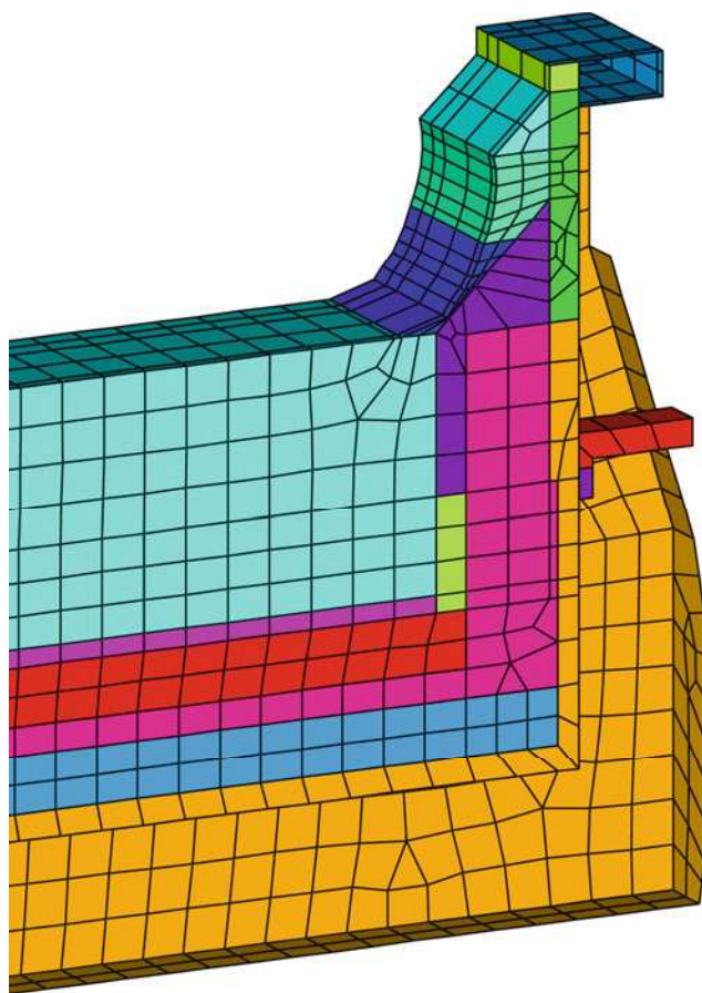
Fig. 3 500 kA cathode side slice model mesh
