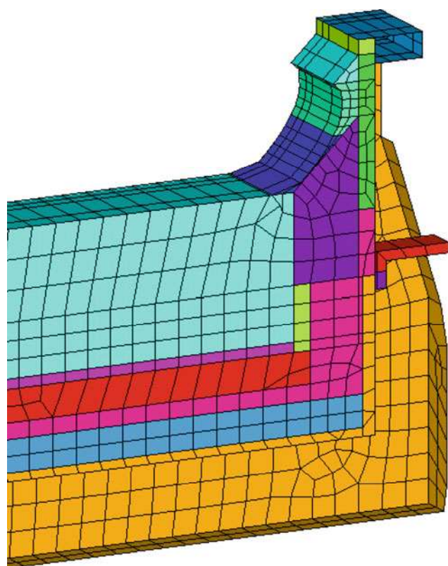
Fig. 1 600 kA cathode side slice model mesh
