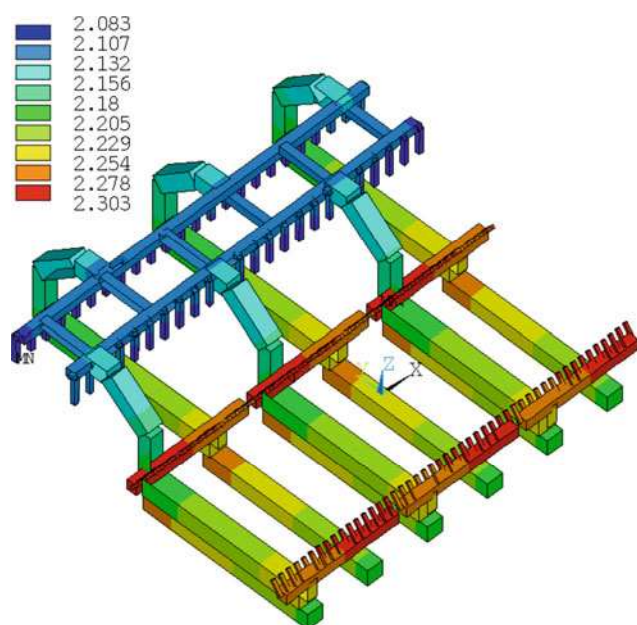
Fig. 5 650 kA model predicted busbar voltage drop
