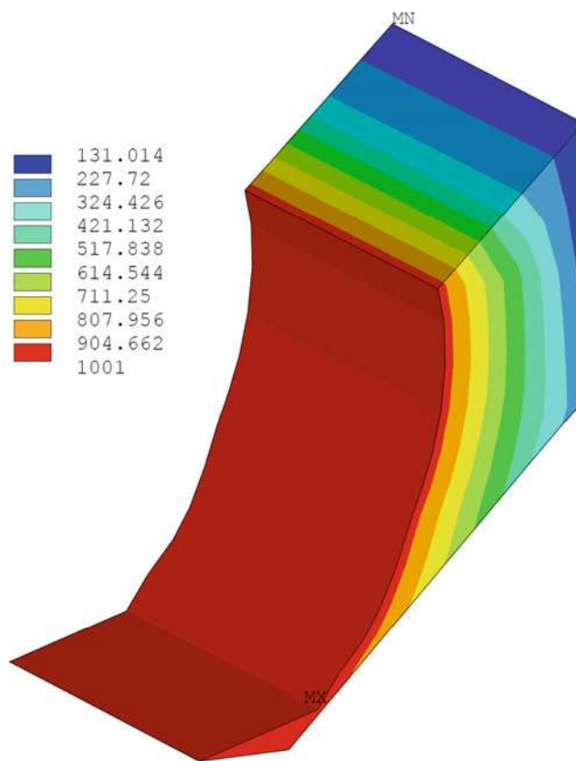
Fig. 4 500 kA model downstream side ledge temperature
