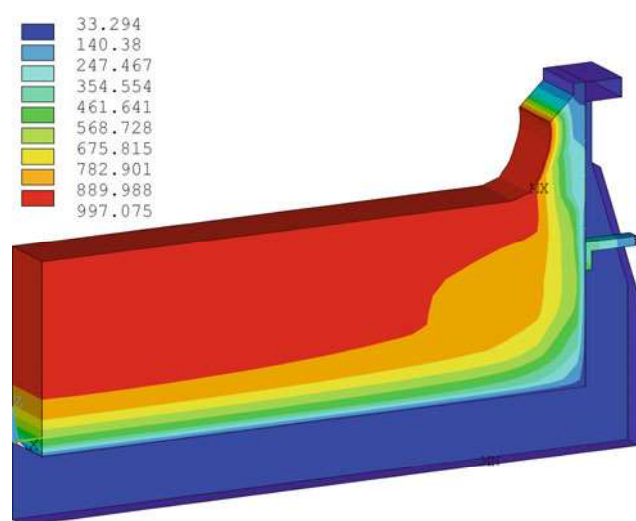
Fig. 7 650 kA cathode side slice model temperature solution
